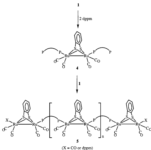
Scheme 2. Reactivity of complex 1 with dpmm
